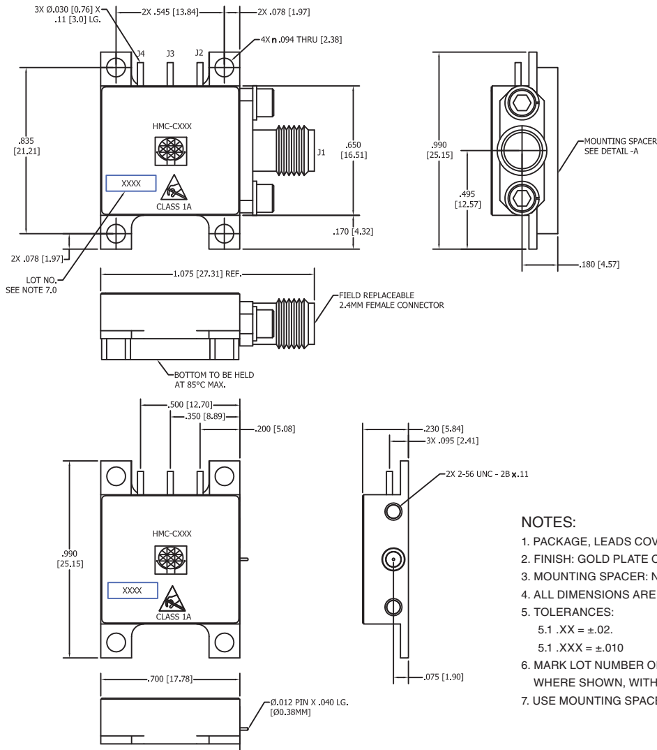
VIEW SHOWN WITH CONNECTOR AND MOUNTING SPACER REMOVED
